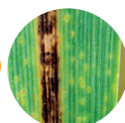
Helminthosporiose
